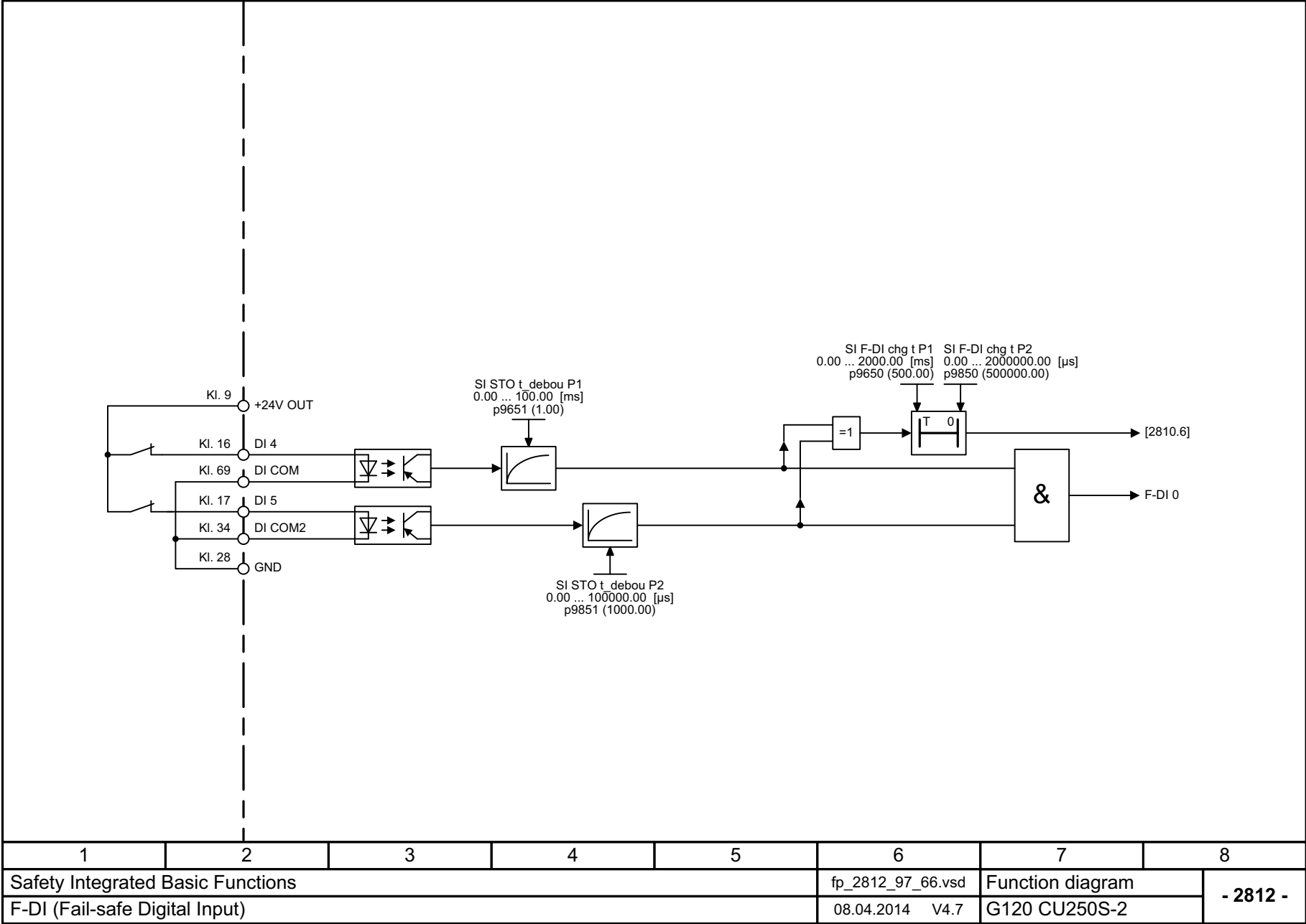
图 3-79 2812 - F-DI (Fail-safe Digital Input)
