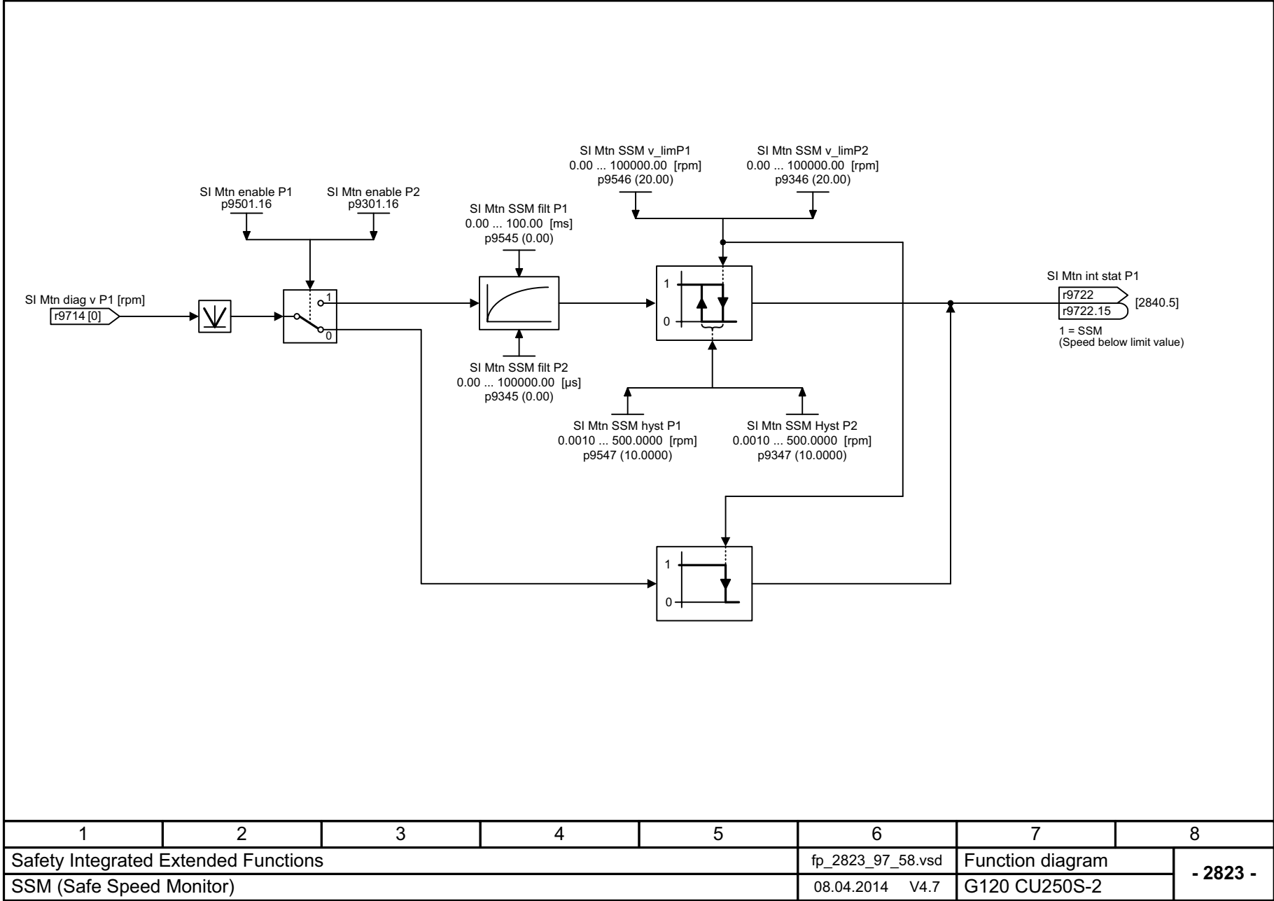
图 3-83 2823 - SSM (Safe Speed Monitor)
